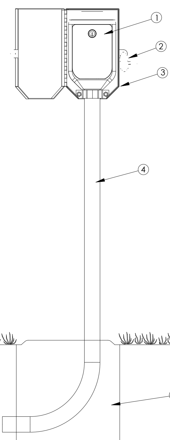
Light energized irrigation controller LEIT 4000 and 4000E with light accessible stainless steel enclosure
