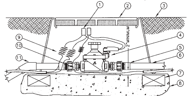
2 150S-150-200 1-1/2" AND 2" REMOTE CONTROL VALVE ASSEMBLY
